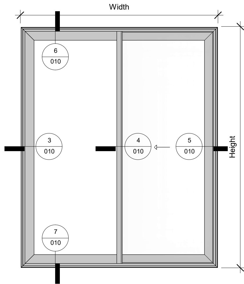
1 Elevation Front 1 : 20
